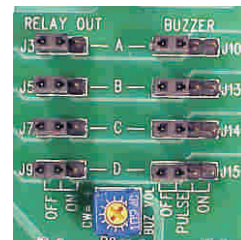
Audible alarm configured by jumpers and volume control on bottom of the unit
